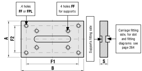
Supports Base BD LXR Used on Rotary nut Groups in supports LXR, DXA, DXR/A and DXR/B. (photo on side of LXR/PS). The same base is also used in the Excellent Groups.
